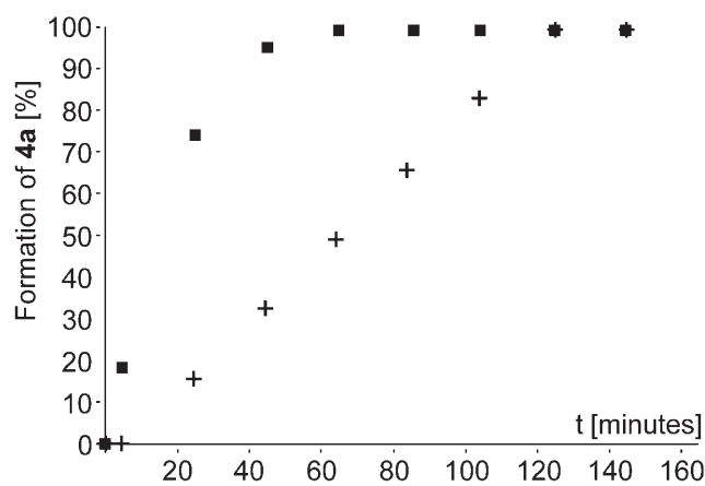
Figure 1. Formation of 4a from 2a and 3 catalyzed by 1 mol % of 1a (■) or 1e (+) in THF- d 8 .
